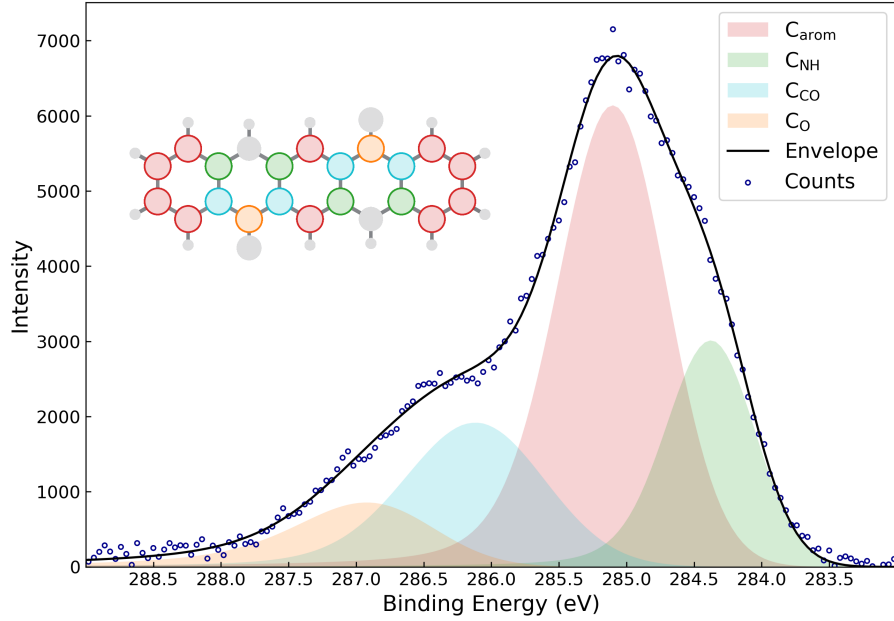
Figure 5.2: C1s XPS spectrum for the \alpha -phase of QA on Ag(100) for a coverage of 1 ML with the experimental data points, the fitted components and the resulting envelope.
