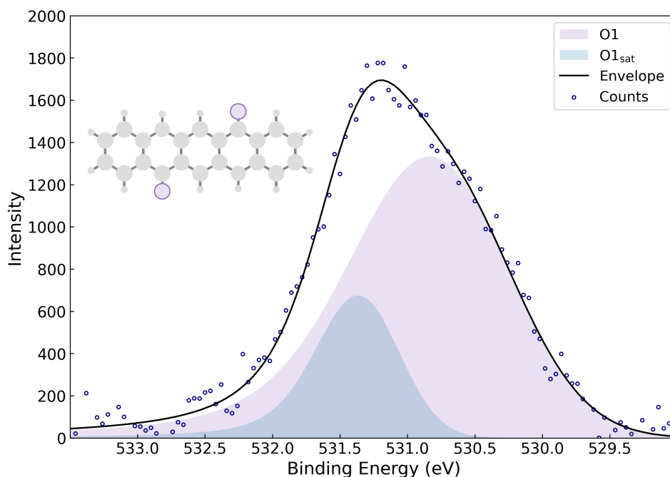
Figure 5.5: O1s XPS spectrum for the \alpha -phase of QA on Ag(100) for a coverage of 1 ML with the experimental data points, the fitted components and the resulting envelope.
