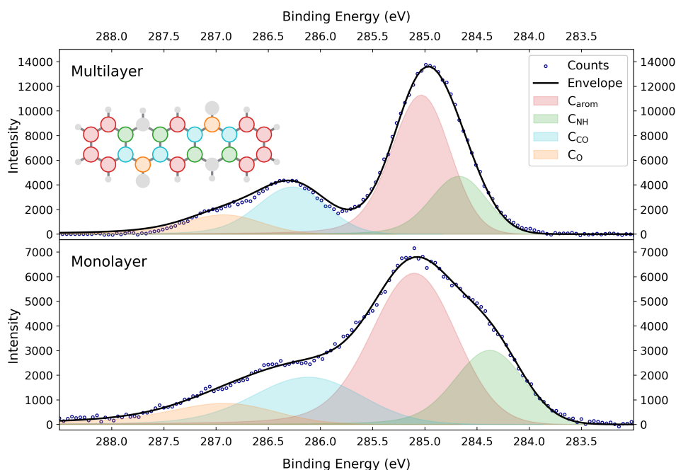
Figure 5.3: C1s XPS spectrum for the \alpha -phase of QA on Ag(100) for a multilayer coverage compared to the XPS spectrum for a coverage of 1 ML with the experimental data points, the fitted components and the resulting envelope.
