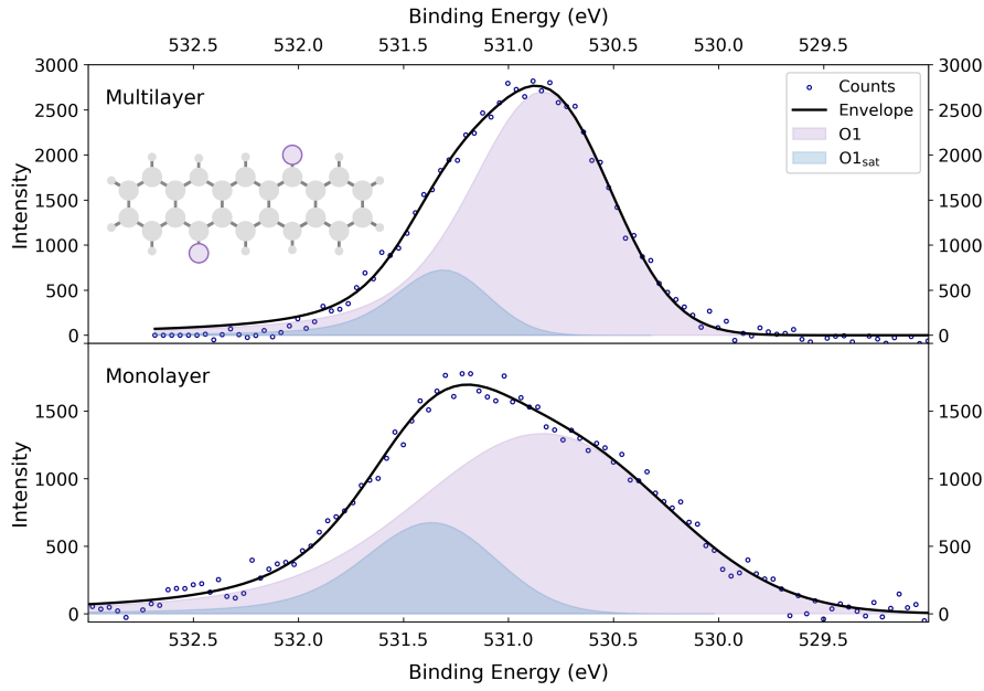
Figure 5.6: O1s XPS spectrum for the \alpha -phase of QA on Ag(100) for a multilayer coverage compared to the XPS spectrum for a coverage of 1 ML with the experimental data points, the fitted components and the resulting envelope.
