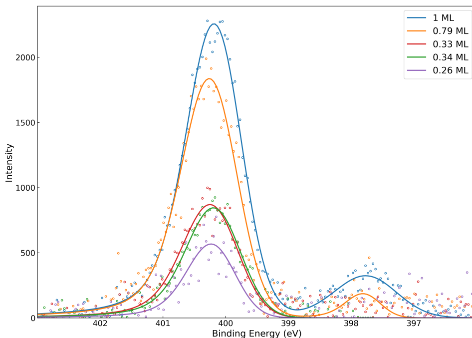
Figure 5.7: Overview of N1s XPS spectra for monolayer preparation of the \alpha -phase of QA on Ag(100) with a coverage between 0.26 ML and 1.00 ML. The line corresponds to the envelope of the fitted peaks and the circles are the measured data points.
