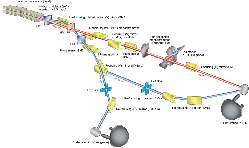
Figure 4.2: Schematic drawing of the I09 endstation of the Diamond Light Source in Didcot, UK. Picture taken from reference [44].
