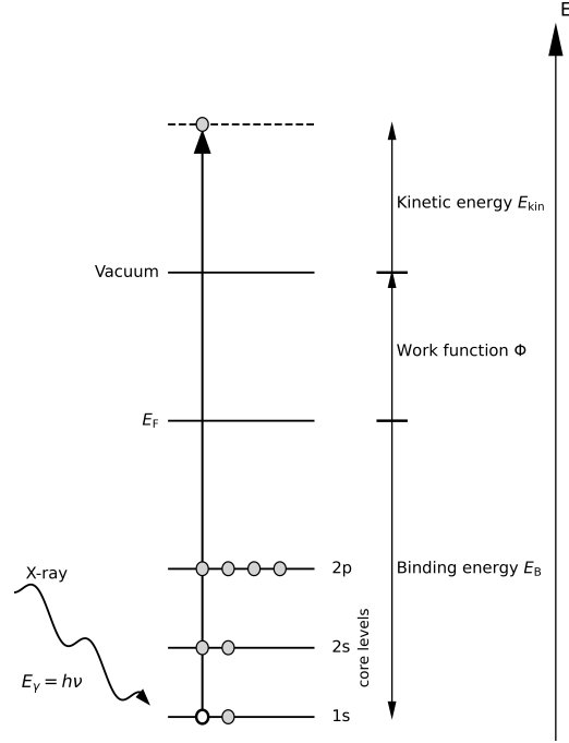
Figure 3.1: Schematic drawing of the photoemission process of an electron in the 1s orbital upon x-ray excitation. The image was adapted using reference [40].
