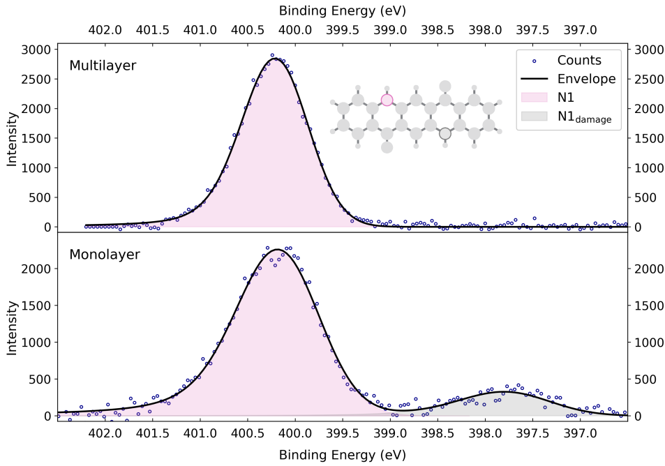
Figure 5.9: N1s XPS spectrum for the \alpha -phase of QA on Ag(100) for a multilayer coverage compared to the XPS spectrum for a coverage of 1 ML with the experimental data points, the fitted components and the resulting envelope.
