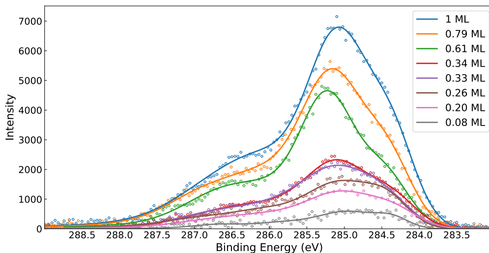
Figure 5.1: Overview of C1s XPS spectra for monolayer preparation of the \alpha -phase of QA on Ag(100) with a coverage between 0.08 ML and 1.00 ML. The line corresponds to the envelope of the fitted peaks and the circles are the measured data points.
