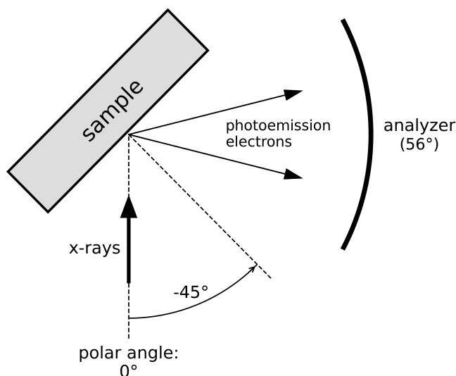
Figure 4.3: Top view of the sample geometries for the XPS measurements at the I09 endstation of the Diamond Light Source in Didcot, UK. Illustrated as in reference [45].
