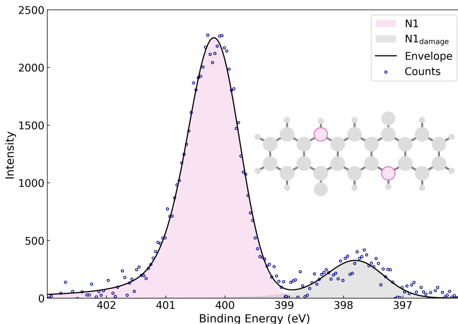
Figure 5.8: N1s XPS spectrum for the \alpha -phase of QA on Ag(100) for a coverage of 1 ML with the experimental data points, the fitted components and the resulting envelope.
