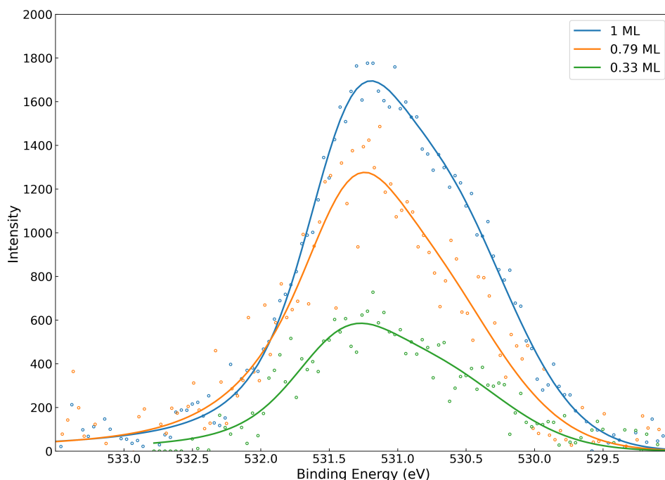
Figure 5.4: Overview of O1s XPS spectra for monolayer preparation of the \alpha -phase of QA on Ag(100) with a coverage between 0.33 ML and 1.00 ML. The line corresponds to the envelope of the fitted peaks and the circles are the measured data points.
